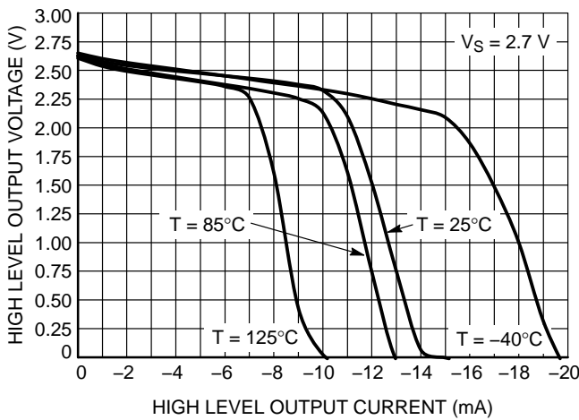
Figure 11. High Level Output Voltage vs. Output Current @ V_S = 2.7 V
